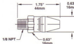
Model 1009 and 1009SS
