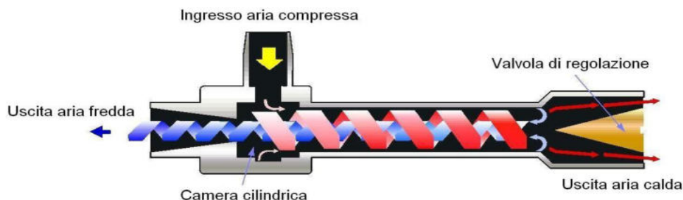
Tubo a vortice small
