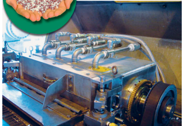
(4) Model 3250 Vortex Tubes cool the cutting knives in this pelletizer to prevent irregular shapes.
