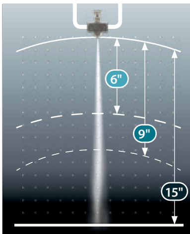
Model: AN8020SS Material: Type 303 Stainless Steel
