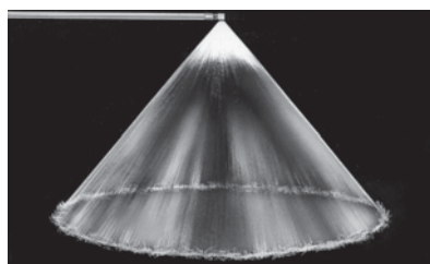
Hollow Cone 80°
