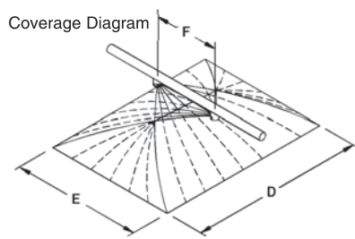
Rectangular Spray
