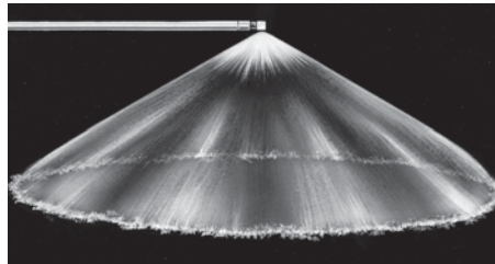
Hollow Cone 120°
