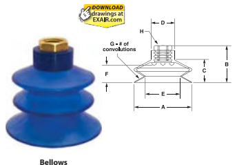
Bellows
