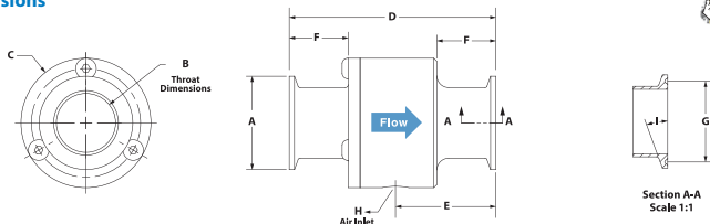
Sanitary Flange Line Vac Dimensions
