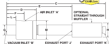
Adjustable Vacuum Generator Dimensions
