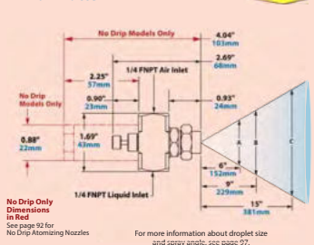
No Drip Only Dimensions in Red See page 92 for No Drip Atomizing Nozzles For more information about droplet size and spray angle, see page 97.
