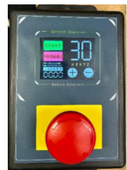
Inverter TG-INVERTER1-TOUCH
