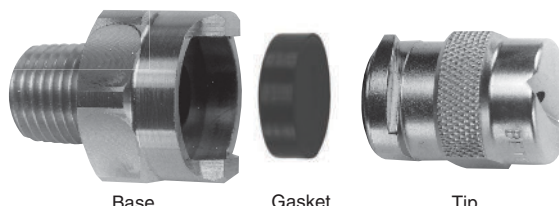
EZNF exploded
